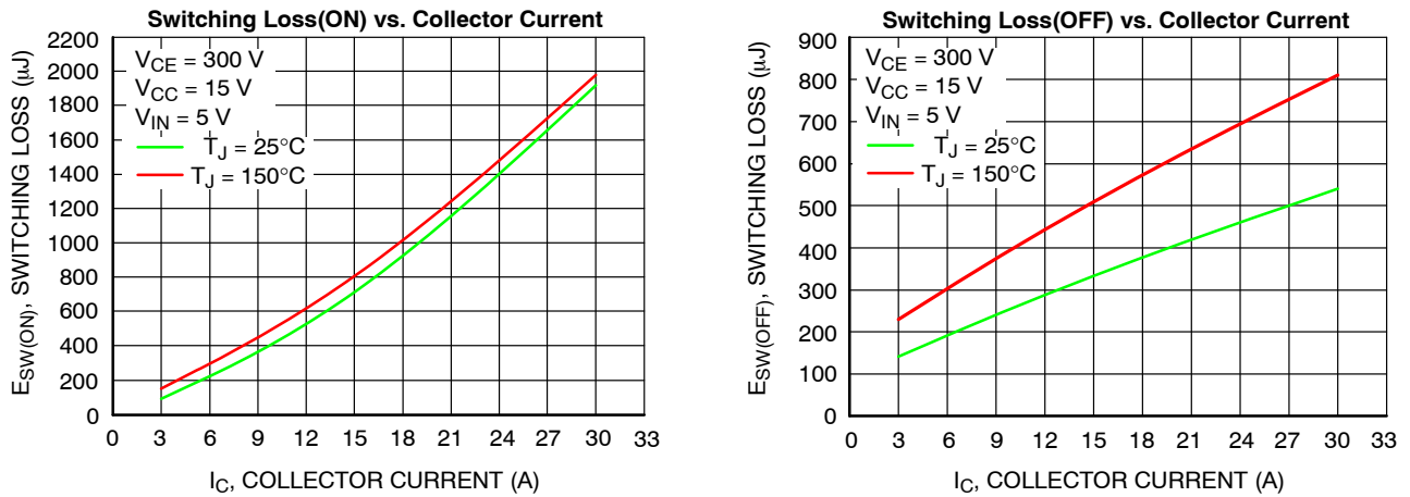
Figure 4. Switching Loss Characteristics
